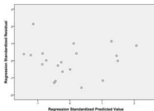
Gambar 2. Scatterplot
